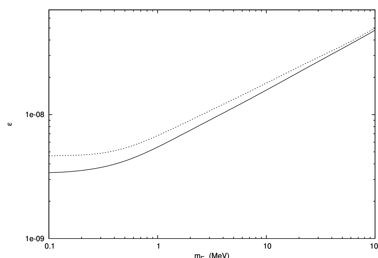
Figure 1: Exclusion limits from \delta N_{\text{eff}}[\text{CMB}] < 0.84 (above solid line) and \delta N_{\text{eff}}[\text{BBN}] < 1 (above dashed line).
