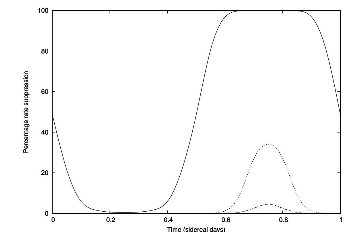
Figure 3: Percentage suppression rate for a detector located at Stawell, for \alpha' = 10^{-2} , |Z'| = 10 , m_{F_2} = 10 GeV, 100 GeV, 1 TeV [solid, dashed, dot-dashed lines], during a sidereal day.
